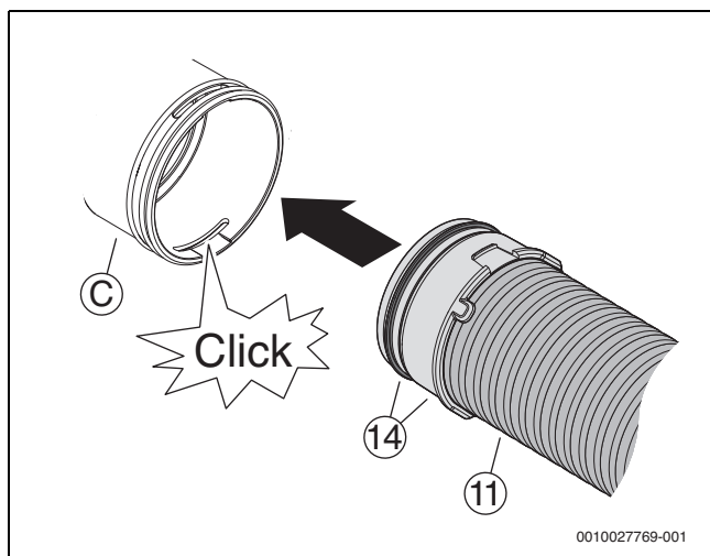
Bild 145 RR 75-1/2 + RRD 75 + VK 160/VK 125 .../VKD-E/RRV 75/RRU 75.../RRB 75-3
